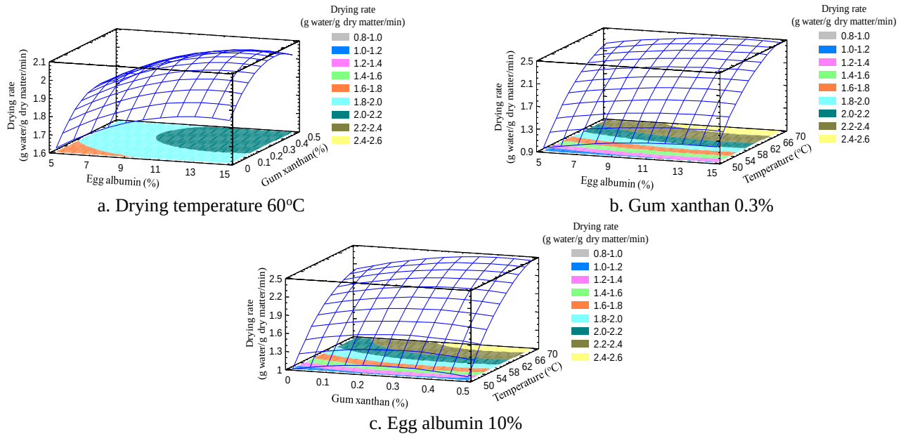
Figure 2: Response surface graph displayed the influence of factors and their interactions on drying rate: a. drying temperature 60°C, b. XG 0.3%, c. EA 10%
