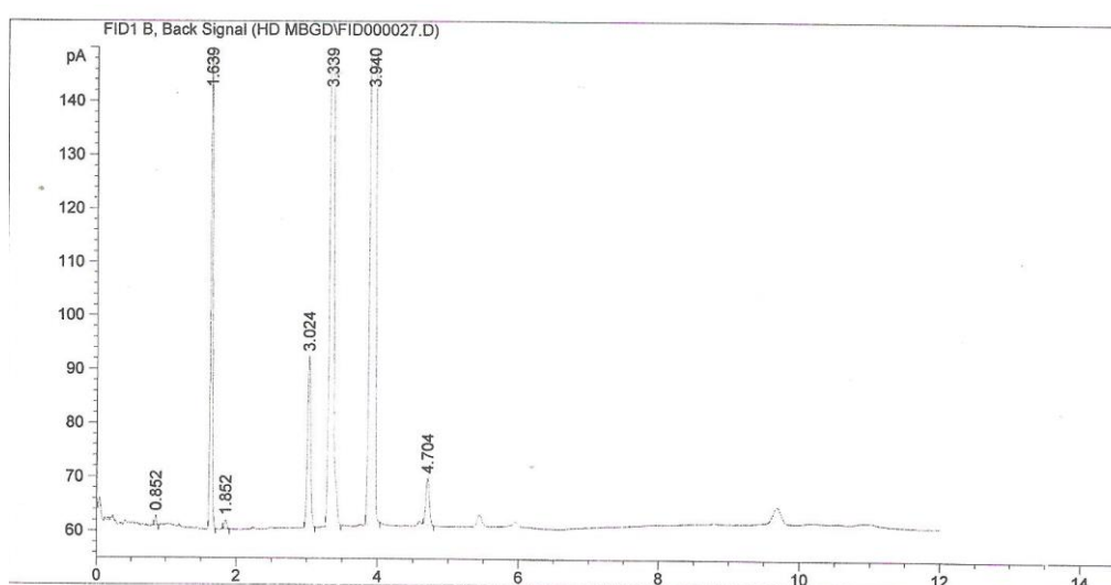
Fig 1. Typical GLC chromatogram showing the separation of FA of cold pressed sunflower seed oil.
